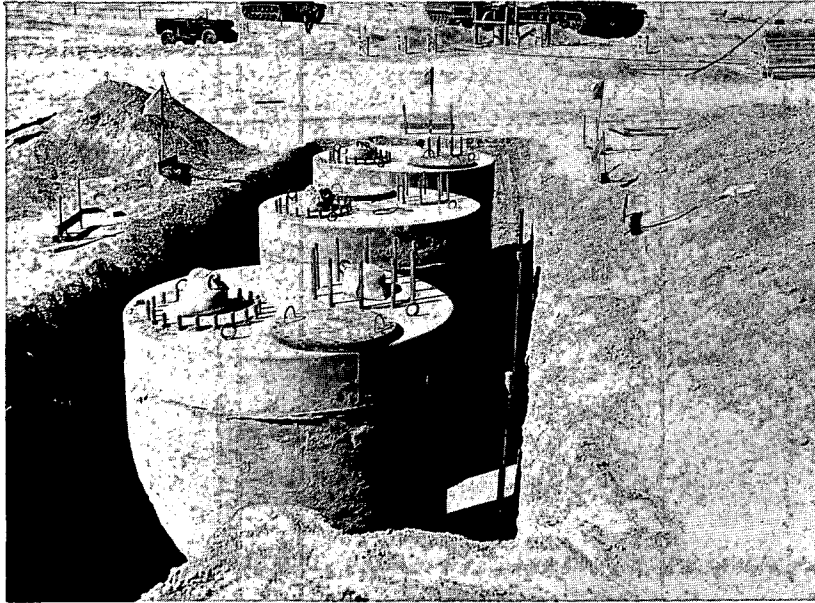
Fig. 1—Test cells in place before backfilling.
